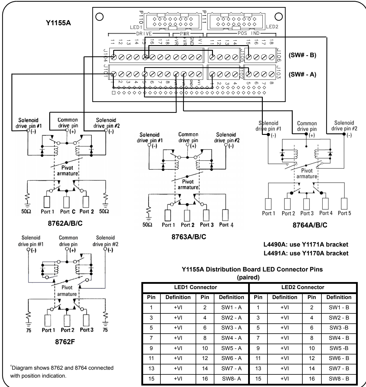
Figure 2-10. Agilent 8762 / 8763 / 8764 Terminal Connections.
