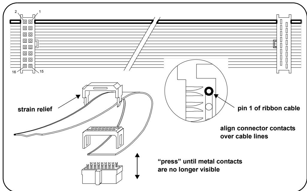
Figure A-7. Y1159A 16-pin to 16-pin Connector Orientation and Cable Routing.
