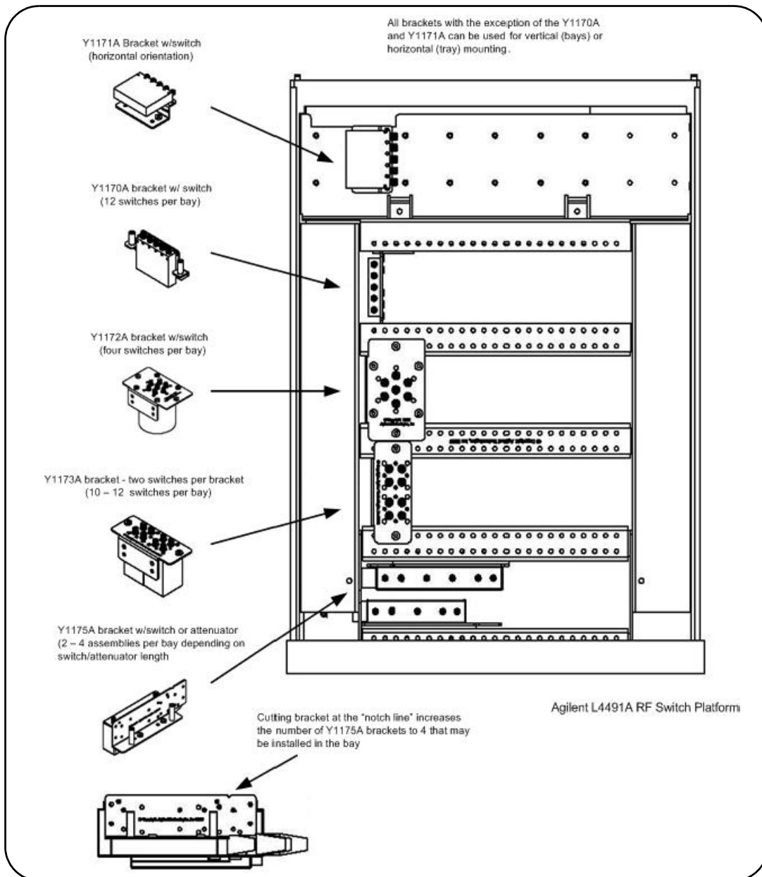
Figure 1-13. Bracket Layout Guidelines.
