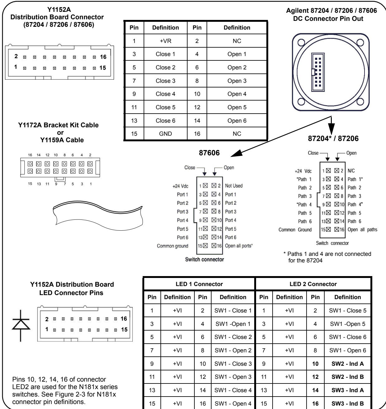
Figure 2-5 Agilent 87204 / 87206 / 87606 Pin Definition and Orientation.
