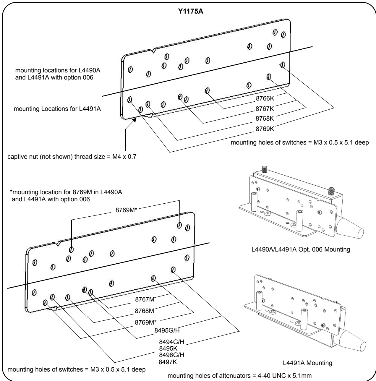
Figure 1-6. Connecting Switches to the Y1175A Bracket.
