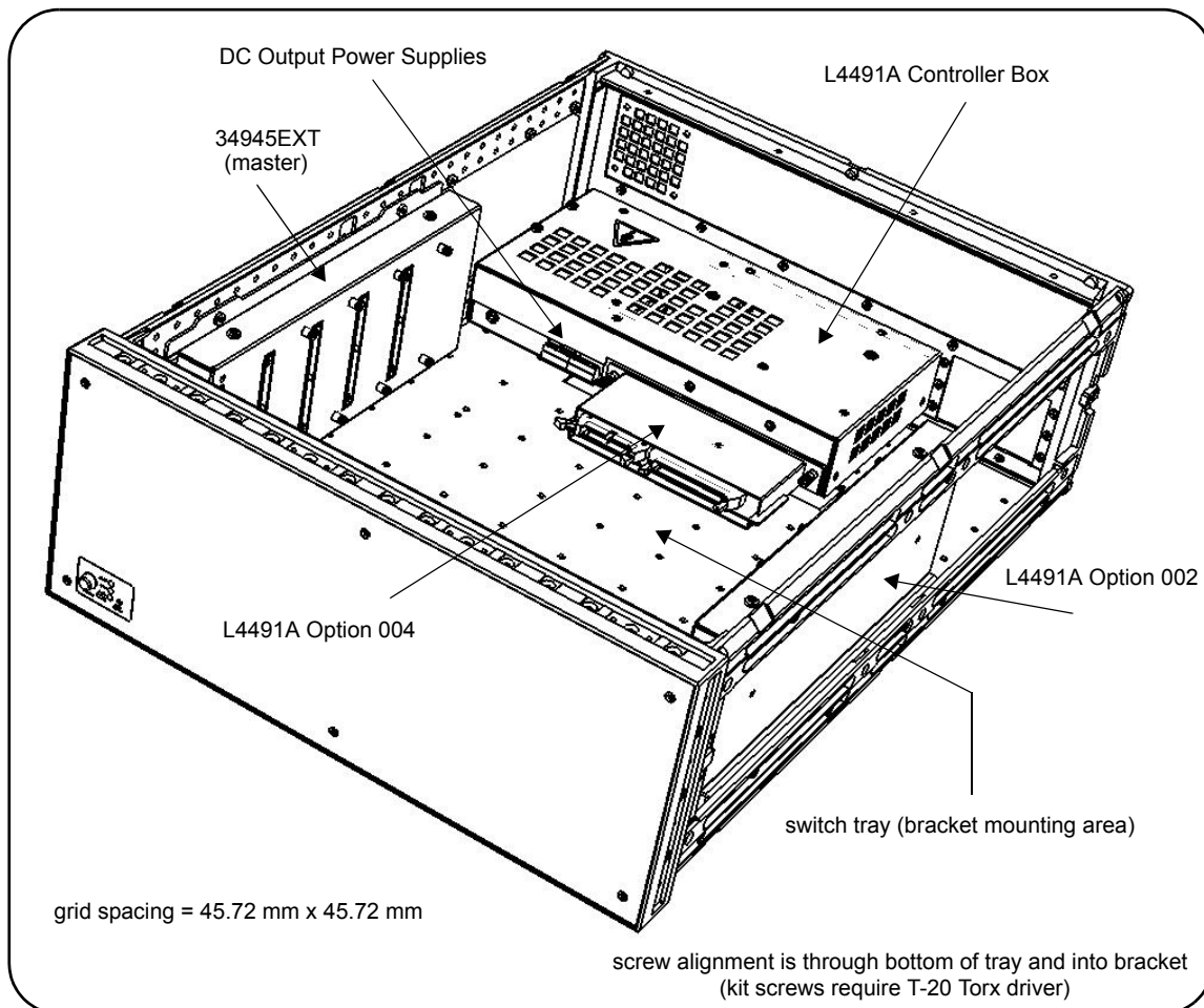
Figure 1-11. L4491A Bottom Switch Tray Option 006.
