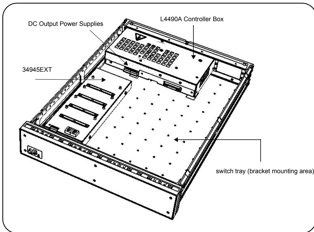
Figure 1-7. L4490A Bracket Mounting Locations.
