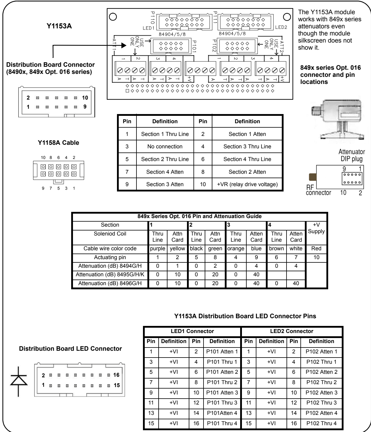
Figure 2-9. Agilent 8494 / 5 / 6 / 7 Attenuator Pin Definitions and Connections.
